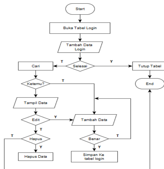
Gambar 5. Flowchart sistem
